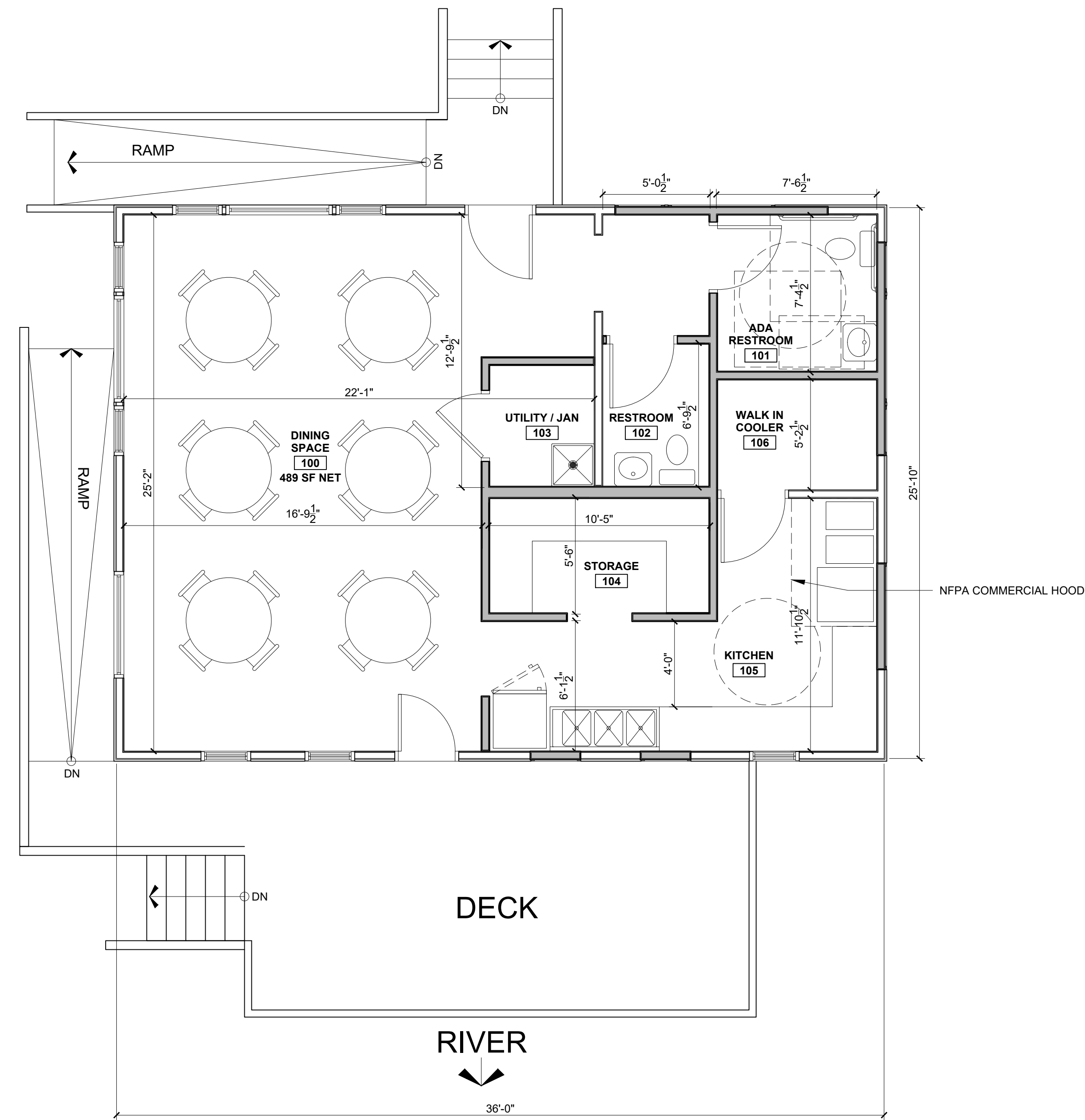
BUILDING FOOTPRINT 930 SF
